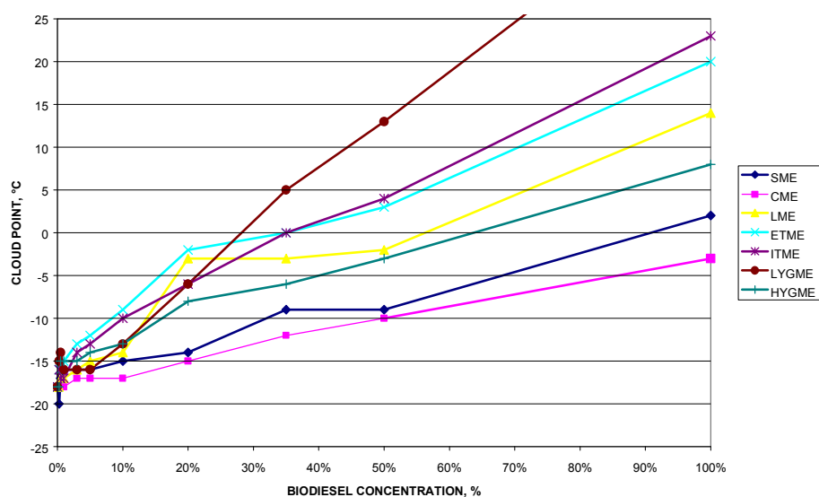
Figure 10. Biodiesel/diesel blend cloud point test results 11
